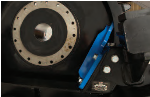
Fully integrated scraper (in blue) for reduced debris build up between the drive wheel and the belt lugs to avoid misalignment and increased belt wear.
